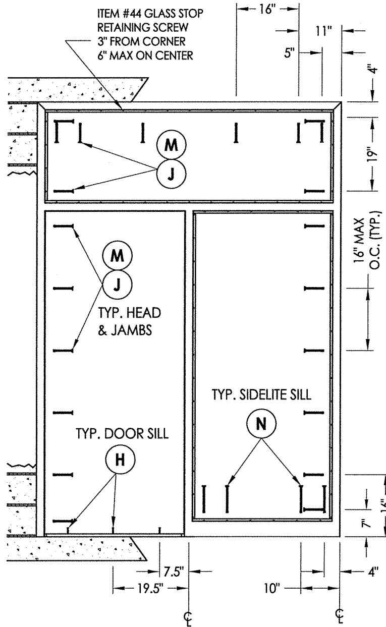
FRAME ANCHORING
