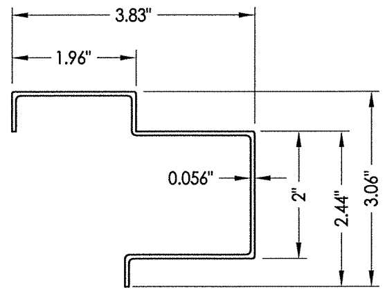
15 MULLION
