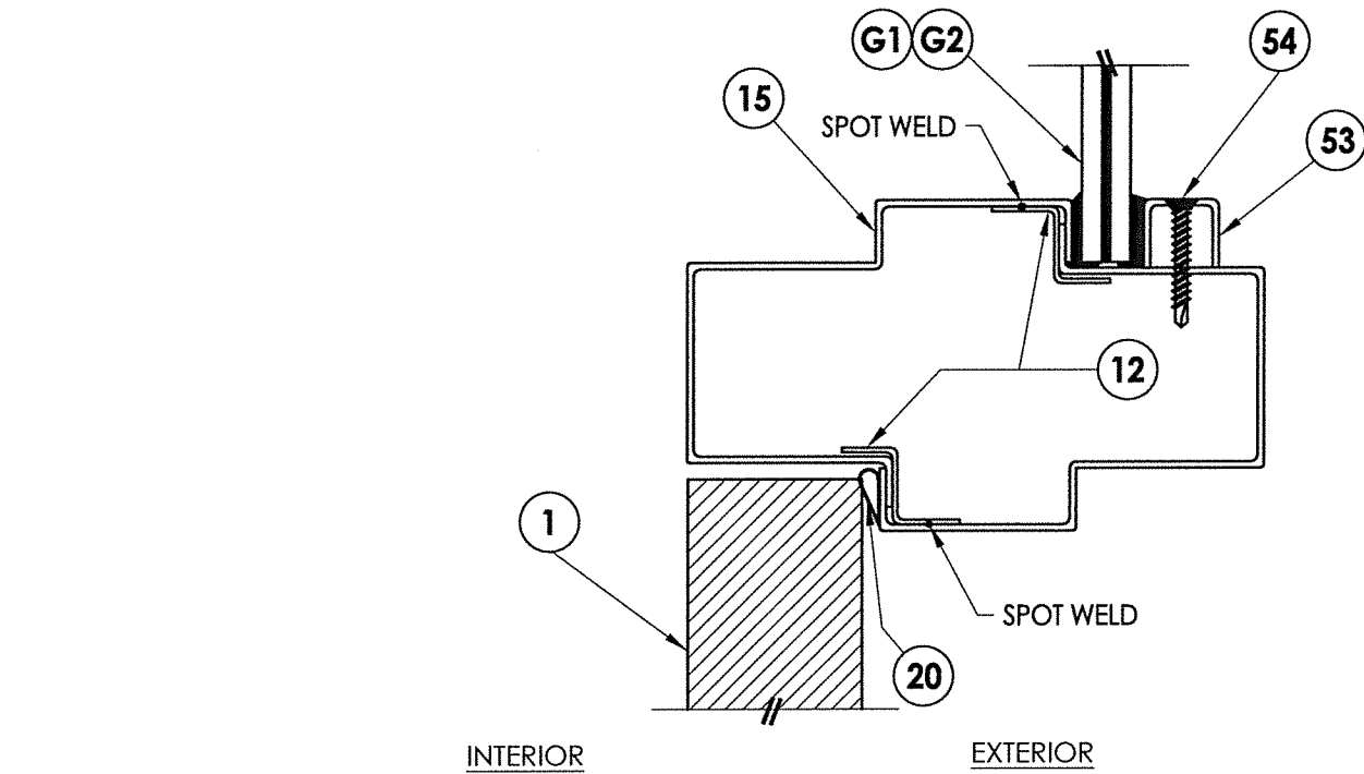
1 4 VERTICAL CROSS SECTION Inswing configuration
